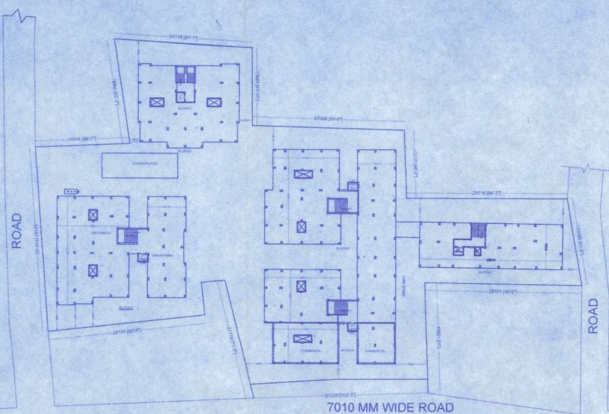
SITE PLAN (BLOCK-A,B,C,D,&E) SCALE:- 1:400
