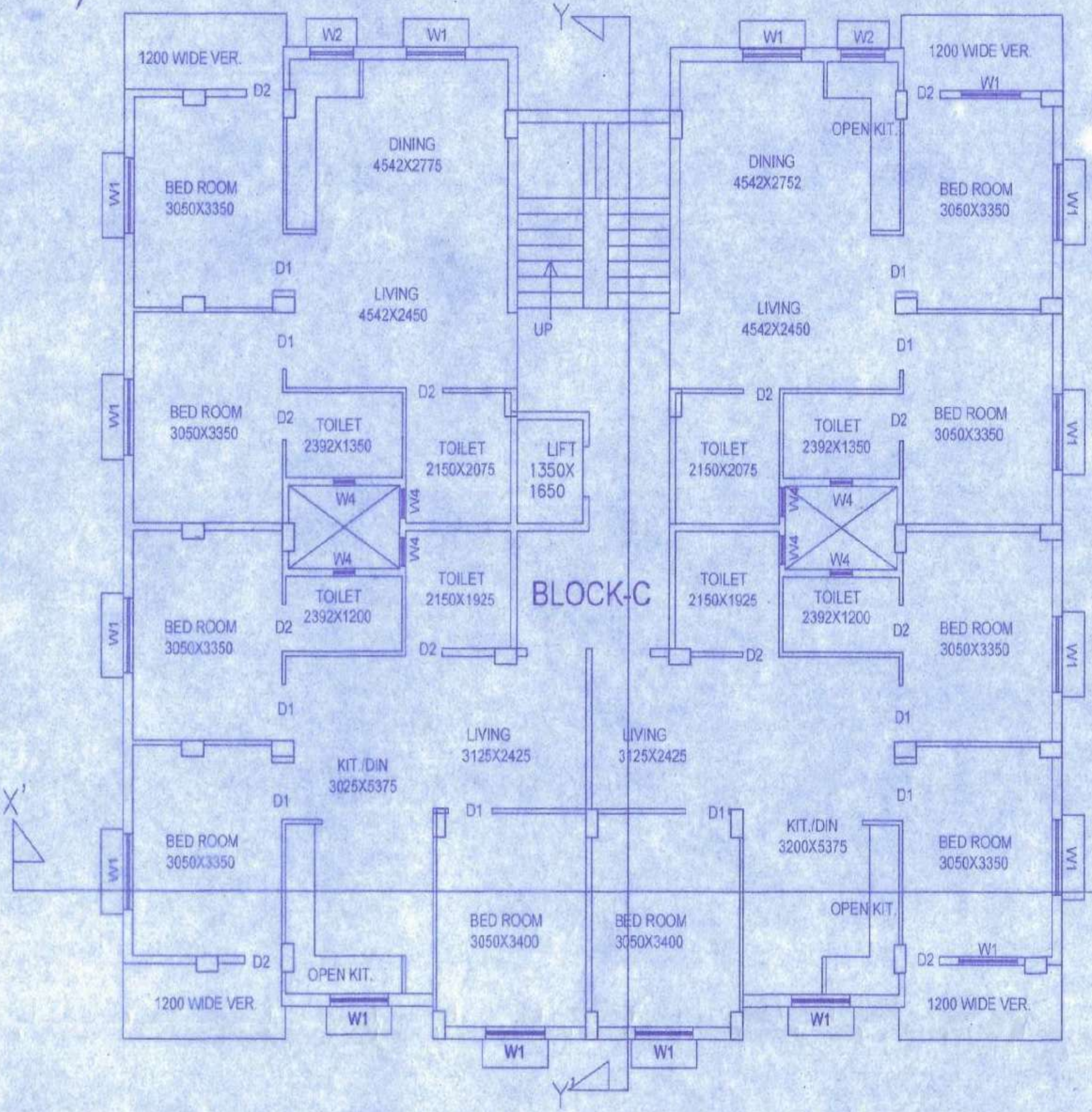
TYPICAL FLOOR PLAN( BLOCK-C) SCALE :- 1:100
