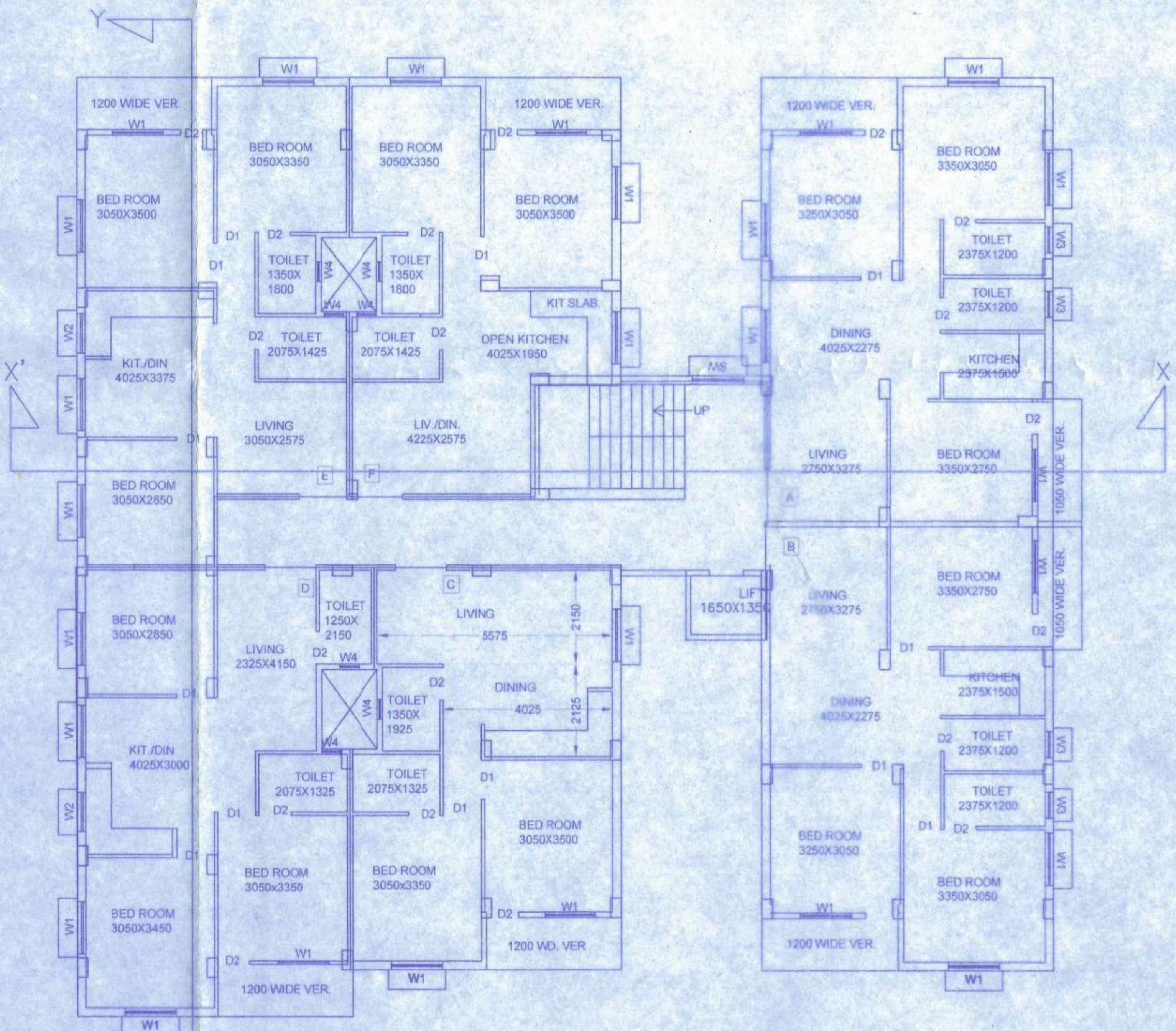
TYPICAL FLOOR PLAN BLOCK-D SCALE :- 1:100
